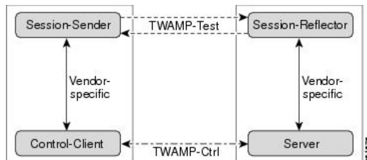
Figure 1: TWAMP Architecture
